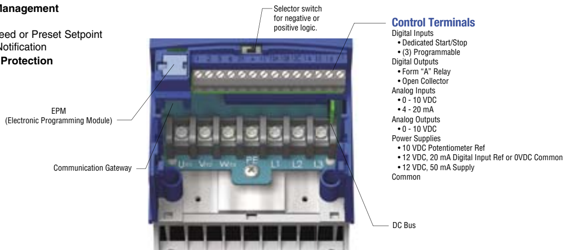
Removable terminal cover and steel conduit plate (not shown). Easy access for control & power wiring. An extra IP21 finger guard ships with every drive.
